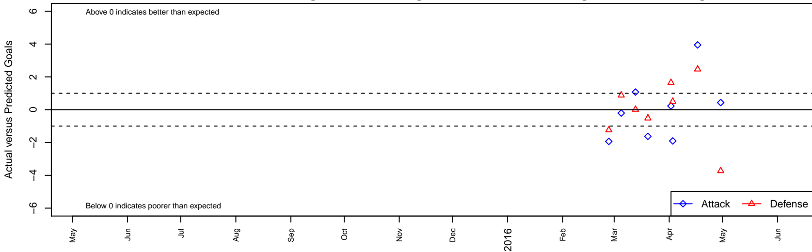
Eclipse FC Aguilitos del America B03 Dots are actual minus expected GF (blue circles) and GA (red triangles). Blue line is smoothed change in attack strength. Red is smoothed change in defense strength.
